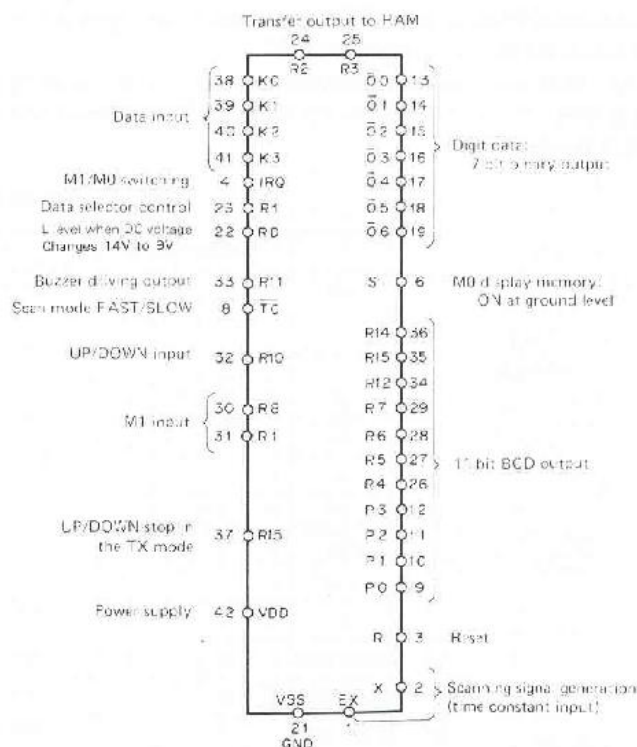
Fig. 14 Microprocessor explanation
