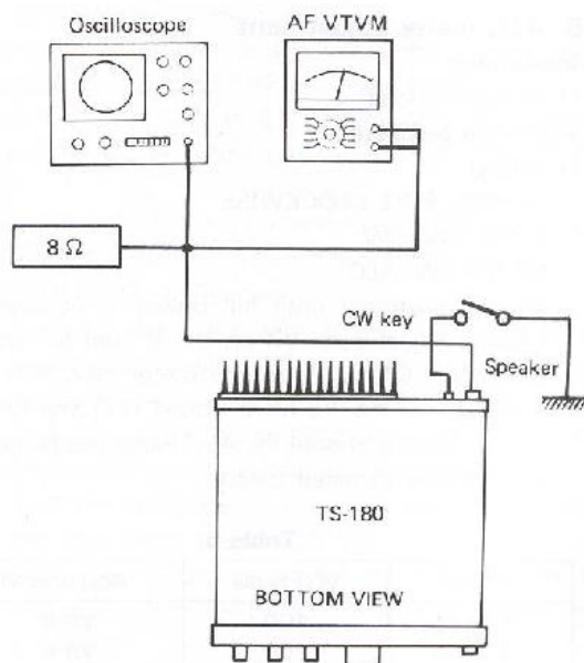
Fig. 43 Side tone adjustment
