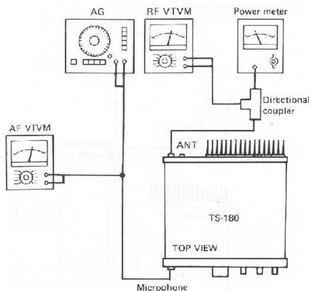
Fig. 42 Carrier point adjustment
