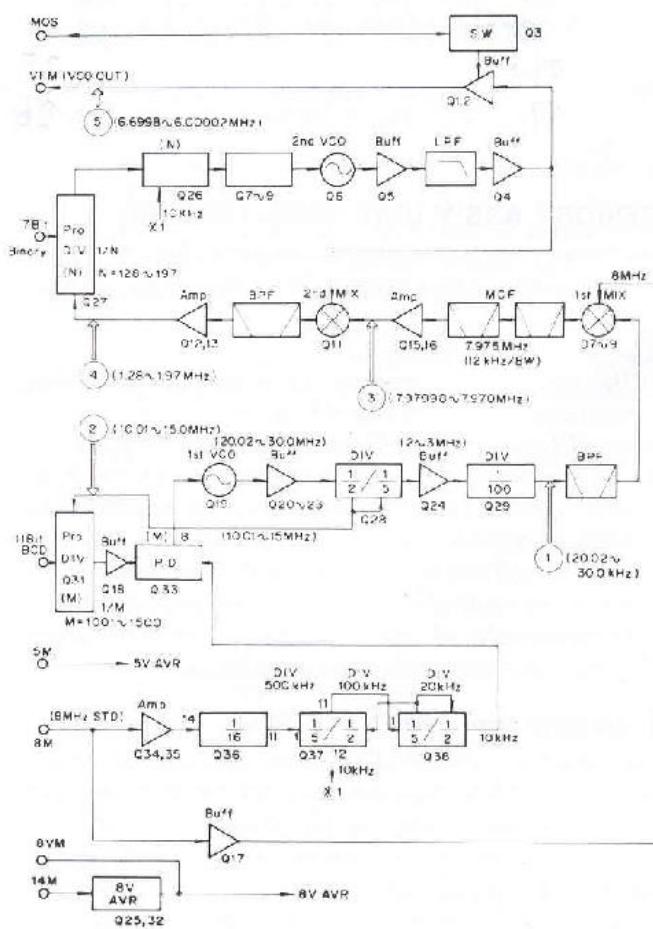
Fig. 15 VCO unit block diagram
